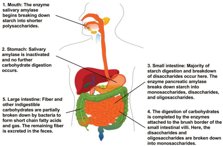
Figure 4.9 Overview of Carbohydrate Digestion
