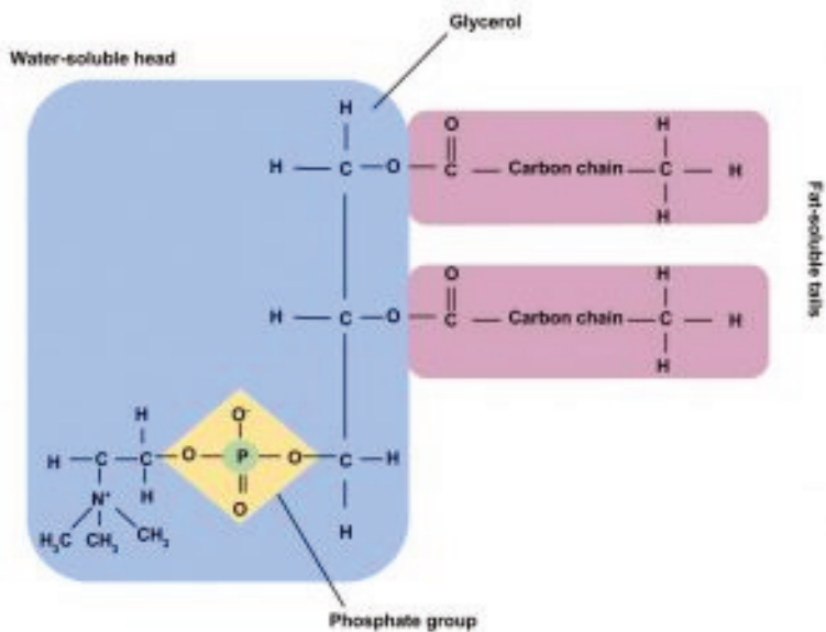
Figure 5.7 The Structure of a Phospholipid
