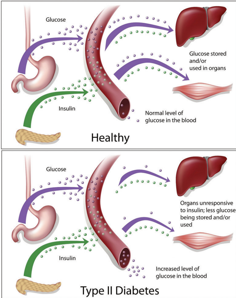
Figure 18.4 Healthy Individuals and Type 2 Diabetes
