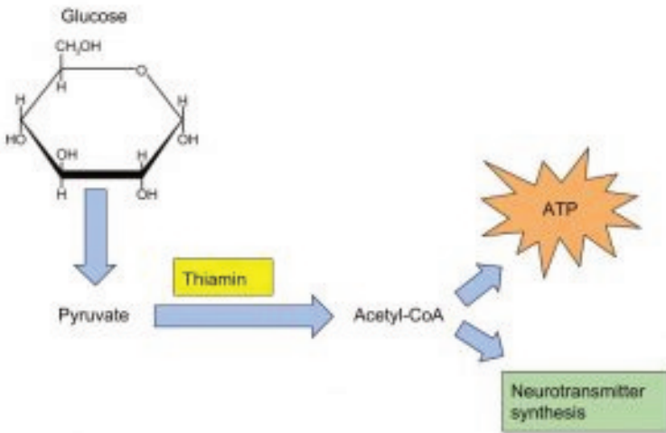
Figure 9.10 The Role of Thiamin
