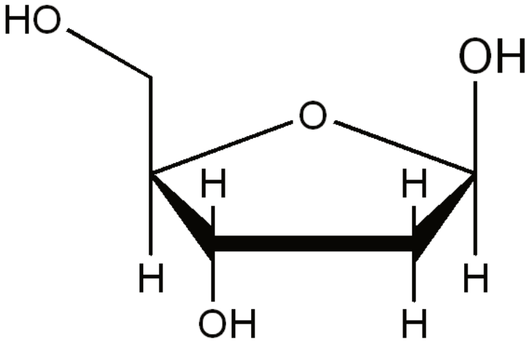
Figure 4.11 Chemical Structure of Deoxyribose
