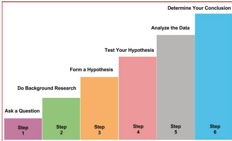
Figure 1.2 Scientific Method Steps
