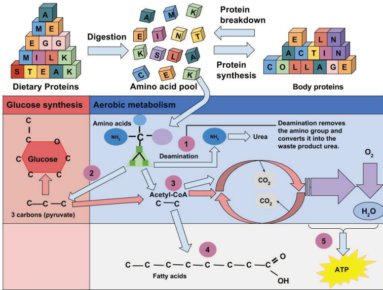
Figure 6.14 Amino Acids Used for Energy
