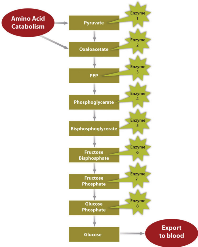
Figure 8.5 Metabolic Pathway of Gluconeogenesis
