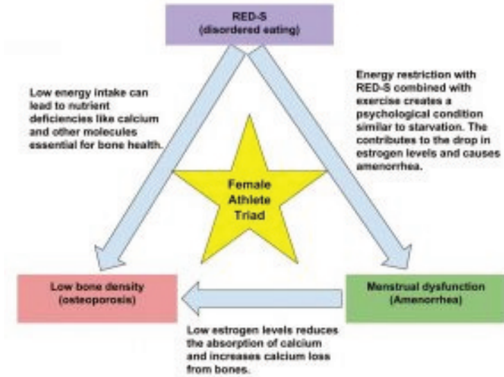
Figure 16.8 The Female Athlete Triad
