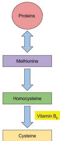
Figure 9.16 Vitamin B 6 Functional Coenzyme Role
