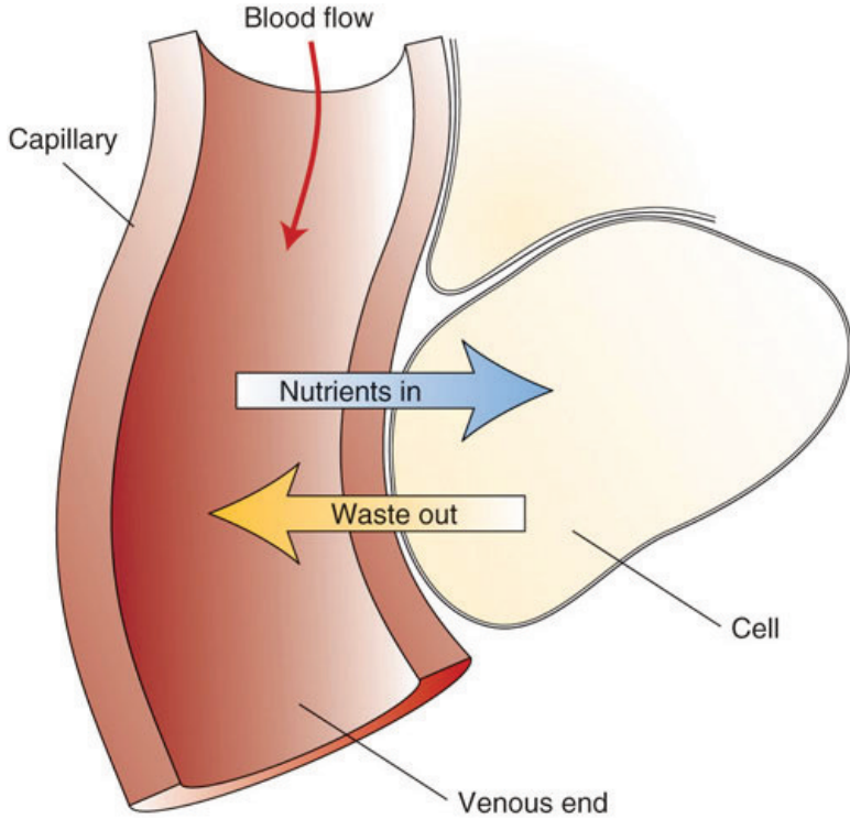
Figure 2.12 Cardiovascular Transportation of Nutrients
