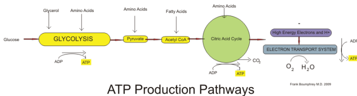
Figure 8.4 ATP Production Pathway
