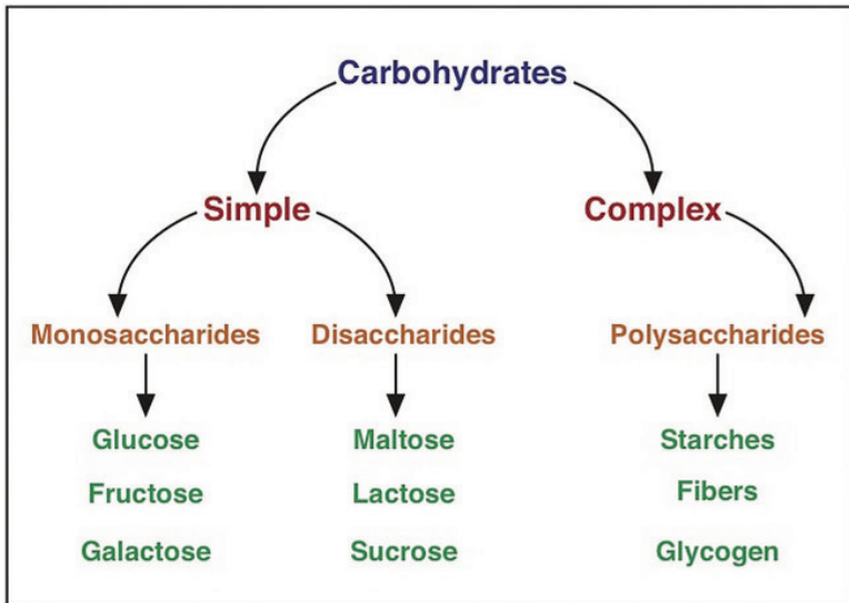
Figure 4.1 Carbohydrate Classification Scheme
