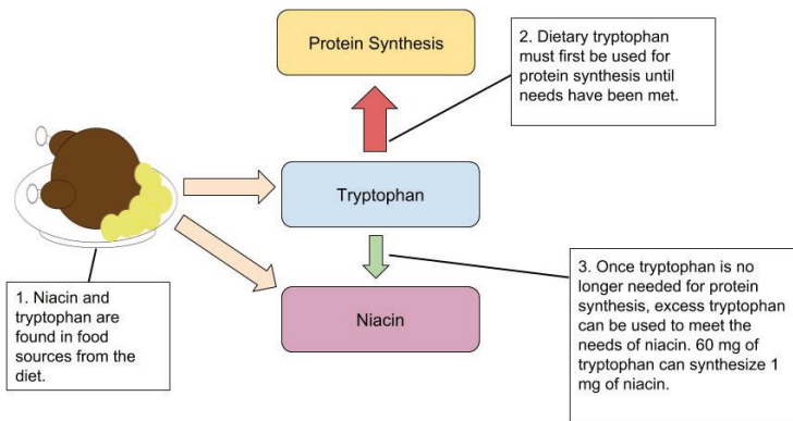
Figure 9.12 Conversion of Tryptophan to Niacin
