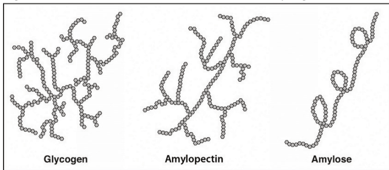
Figure 4.4 Structures of the Plant Starches and Glycogen
