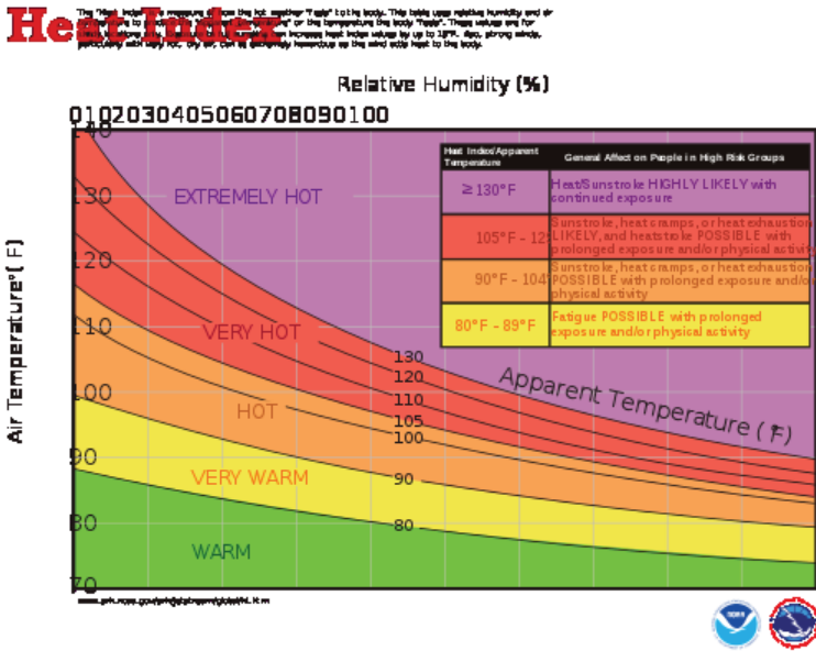
Figure 16.10 The Heat Index
