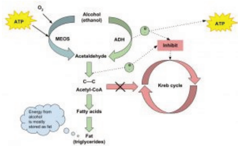
Figure 7.1 Alcohol Metabolism Summary
