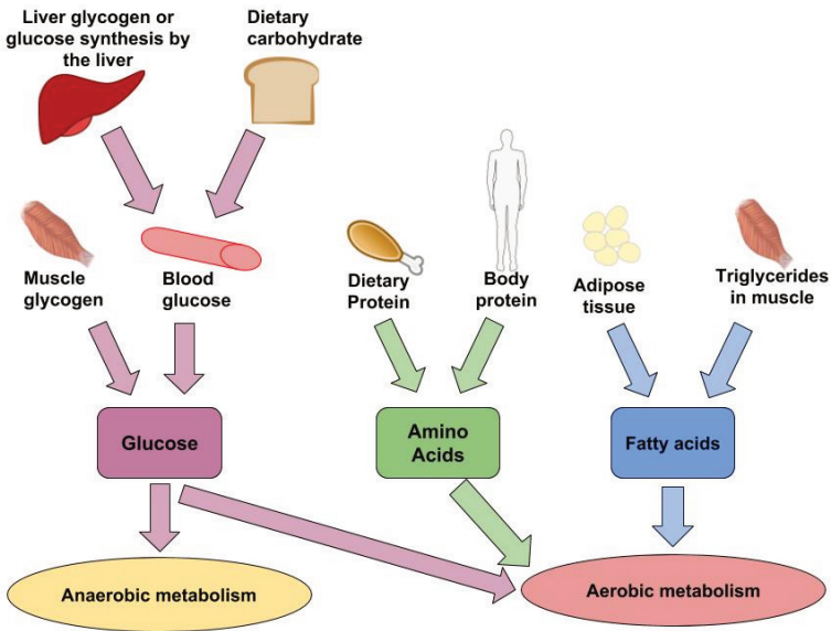
Figure 16.5 Fuel Sources for Anaerobic and Aerobic Metabolism
