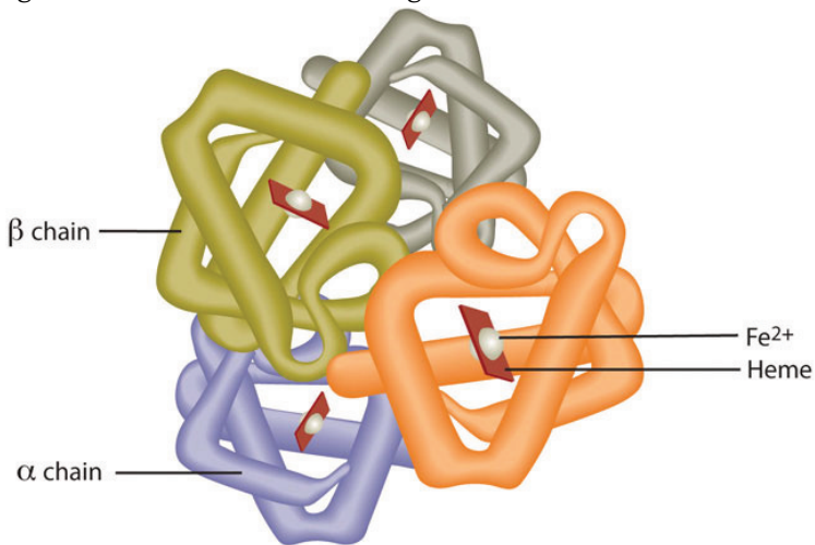
Figure 11.2 The Structure of Hemoglobin
